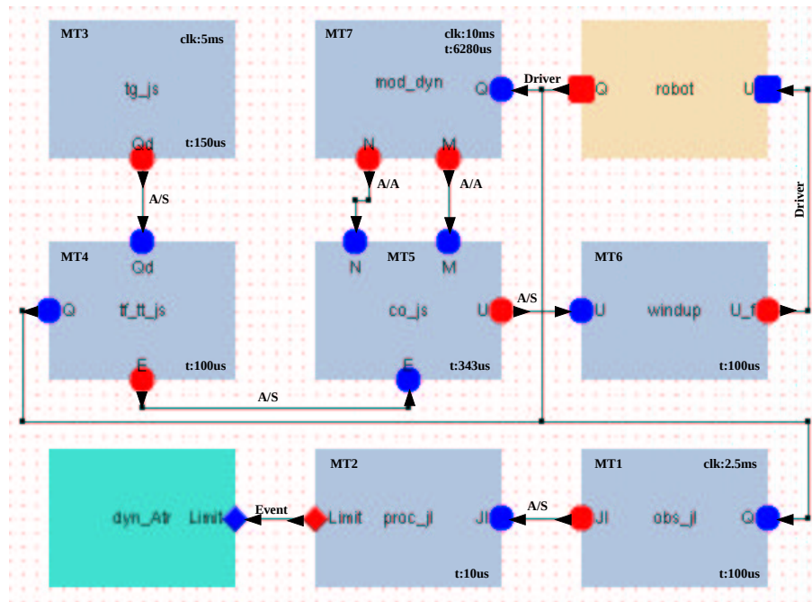
Figure 12: Computed-torque robot controller
