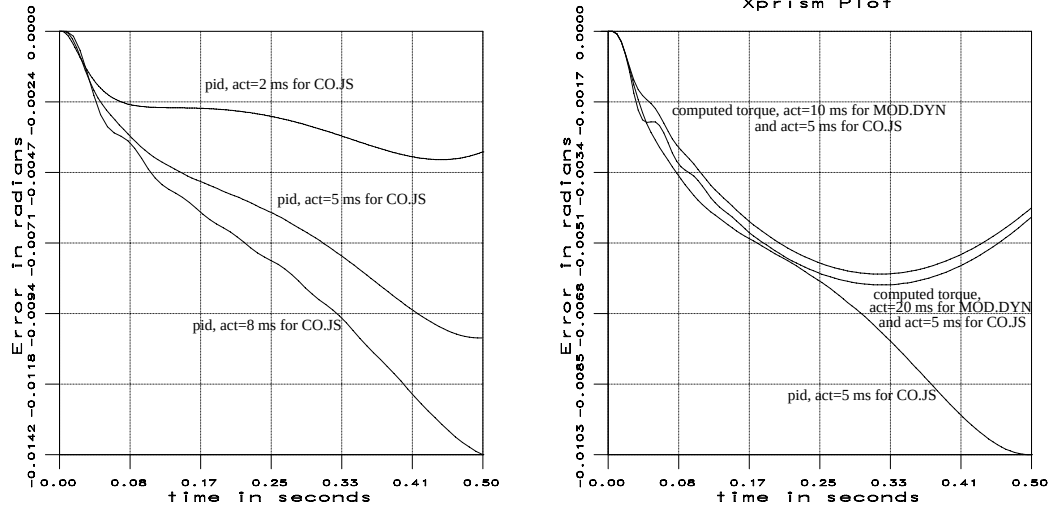
Figure 7: Tracking errors: (a) PID control – (b) Computed torque control
