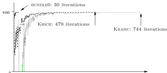
Fig. 2.3. TSP: Kelley vs. bundle on bays29
