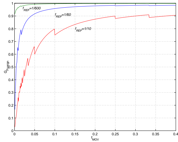
Figure 8: G_{foreign} for different values of f_{reqREF}
